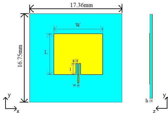
FIGURE 4. Geometry of the proposed element.
