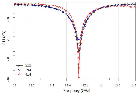
FIGURE 6. The result of the antenna array impedances matching characteristics.
