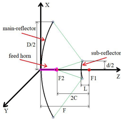
FIGURE 2. Geometry of the Cassegrain antenna system.
