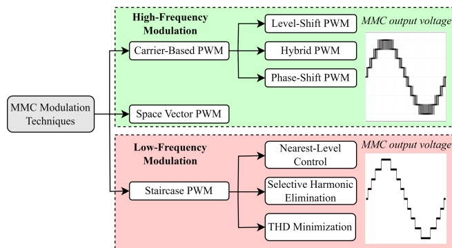
FIGURE 1. Conventional MMC modulation techniques.
