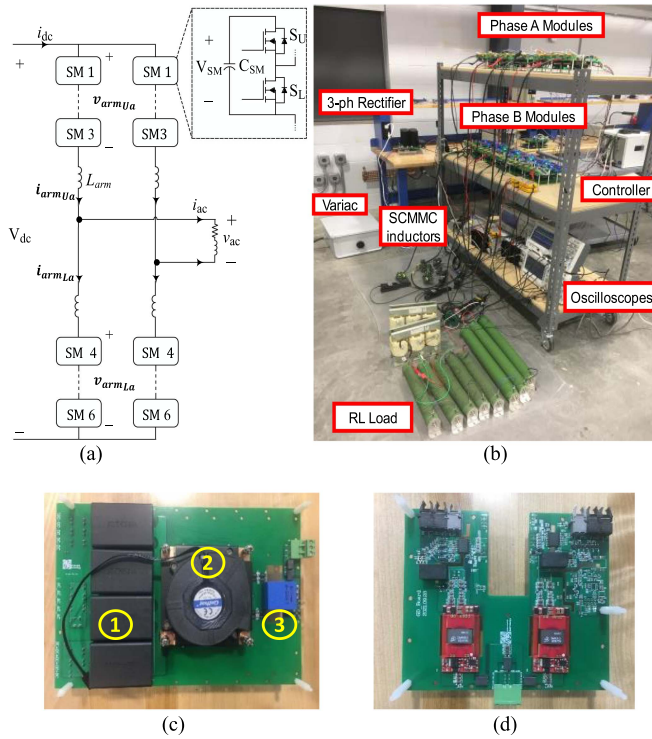
FIGURE 16. 2-phase leg, 4-level SCMMC prototype setup (a) circuit diagram, (b) experimental setup, and (c) SM power board; 1: SM capacitors, 2: SiC module with cooling fan and heat sink, 3: voltage monitoring, and (d) gate-driver board.
