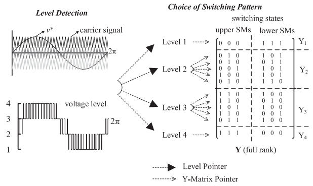
FIGURE 3. YMM of a 4-level SCMMC.
