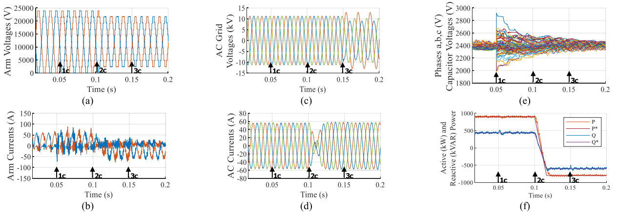
FIGURE 15. Closed loop grid connected mode simulation results of SMM with LFRS; the arrows annotate the simulated events presented in Table 4 (a) phase a arm voltages, (b) phase a arm currents, (c) AC grid voltages, (d) AC currents, (e) all SM capacitor voltages, and (f) active and reactive powers.
