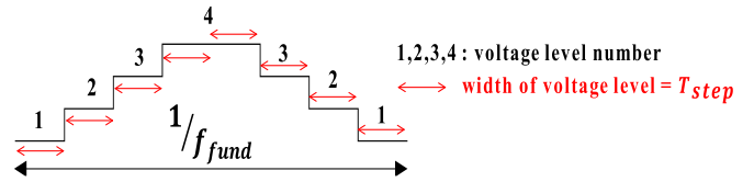
FIGURE 11. Staircase output phase voltage waveform of 4-level SCMMC.
