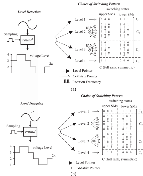
FIGURE 5. SMM for 4-level SCMMC with (a) high-frequency rotation scheme (HFRS) and (b) low-frequency rotation scheme (LFRS).
