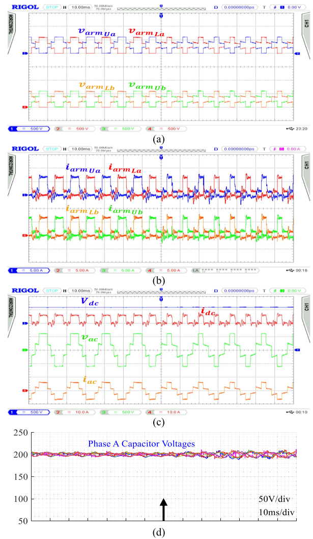
FIGURE 17. 2-ph 4-level SCMMC experimental results under SMM with LFRS (arrow indicates modulation index change from 1 to 0.7) (a) arm voltages, (b) arm currents, (c) ac and dc voltage and currents, and (d) capacitor voltages.
