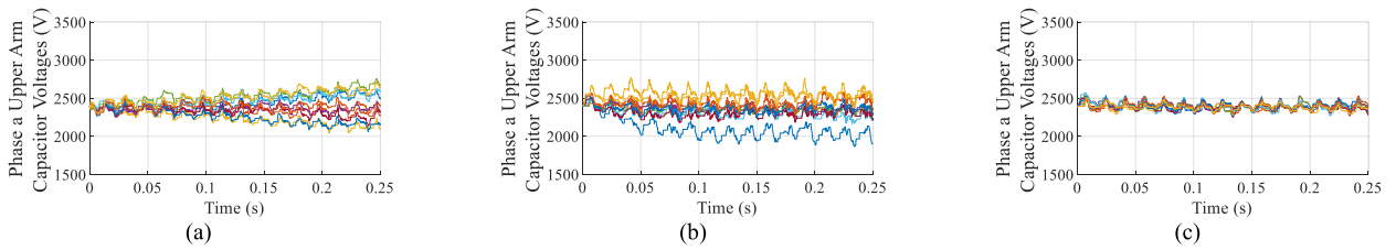
FIGURE 13. Phase a upper arm capacitor voltages with (a) non-full rank symmetric matrix, (b) full rank non symmetric Y-matrix Y , and (c) full rank symmetric C-matrix C (proposed).
