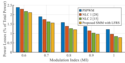
FIGURE 19. Power loss comparison versus modulation index.
