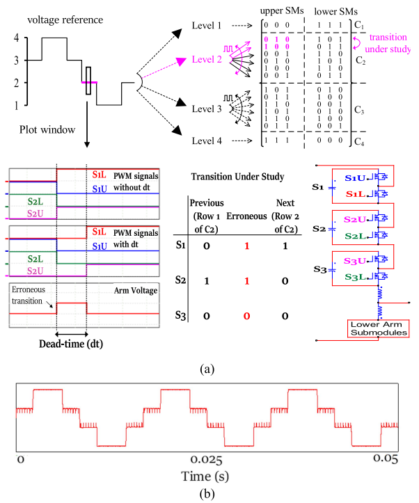
FIGURE 6. Dead-time effect with the high-frequency rotation scheme (HFRS) on a 4-level SCMMC (a) phenomenon and (b) resulting distortions in ac voltage.
