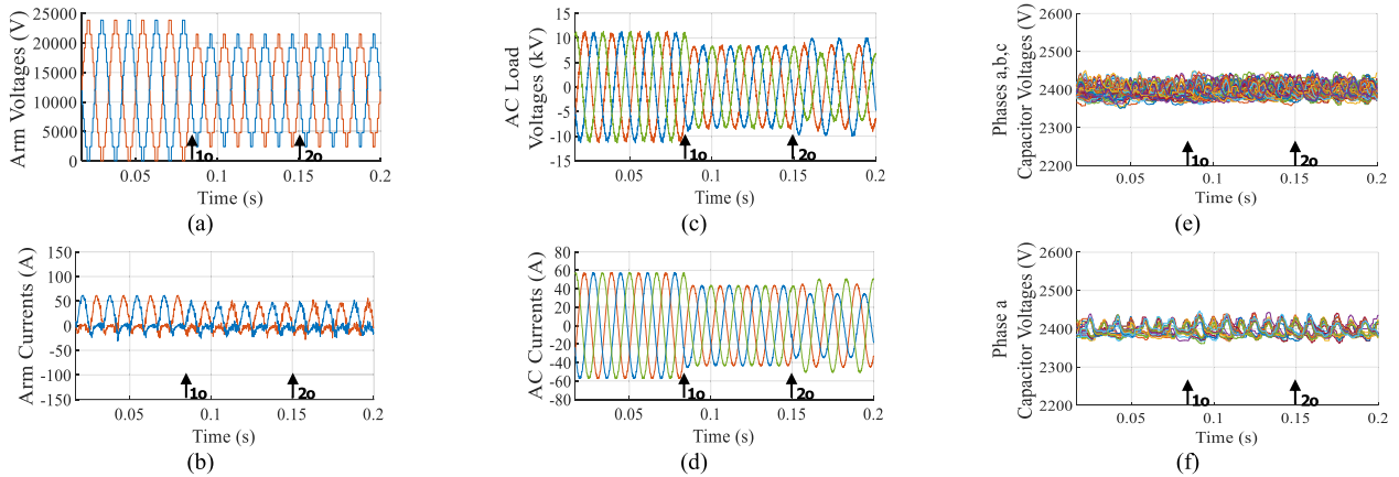
FIGURE 14. Open loop simulation results of SMM with LFRS; the arrows annotate the simulated events presented in Table 3 (a) phase a arm voltages, (b) phase a arm currents, (c) AC load voltages, (d) AC currents, (e) all SM capacitor voltages, and (f) phase a capacitor voltages.
