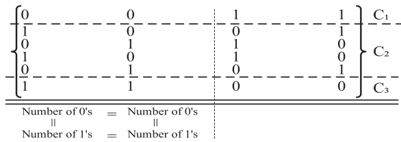
FIGURE 7. Symmetry features of the switching matrix C of a 3-level MMC.
