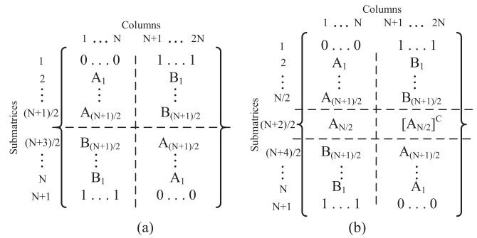
FIGURE 8. Structure of the intermediate switching matrix C' for (a) even level SCMMC and (b) odd level SCMMC.
