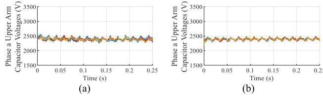
FIGURE 12. Phase a upper arm capacitor voltages with SMM (a) LFRS and (b) HFRS f_{rot} = 6 kHz.
