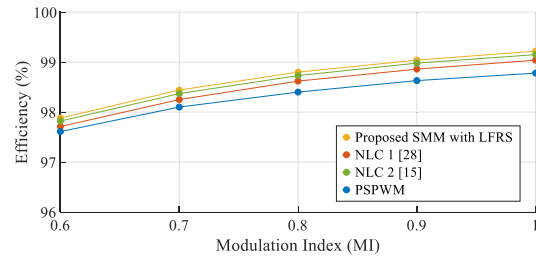
FIGURE 20. Efficiency comparison versus modulation index.
