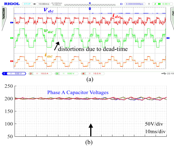
FIGURE 18. 2 – ph 4 – level SCMMC experimental results under SMM with HFRS (arrow indicates modulation index change from 1 to 0.7) (a) ac and dc voltages and currents; (b) capacitor voltages.
