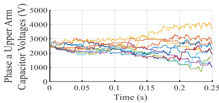
FIGURE 4. SM capacitor voltages under YMM with staircase output voltage.
