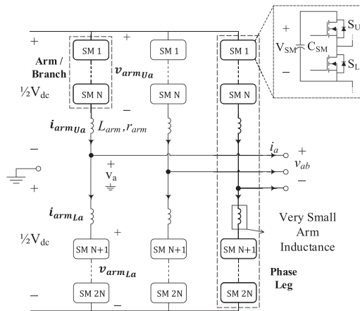
FIGURE 2. 3-phase (N + 1) -level SCMMC.
