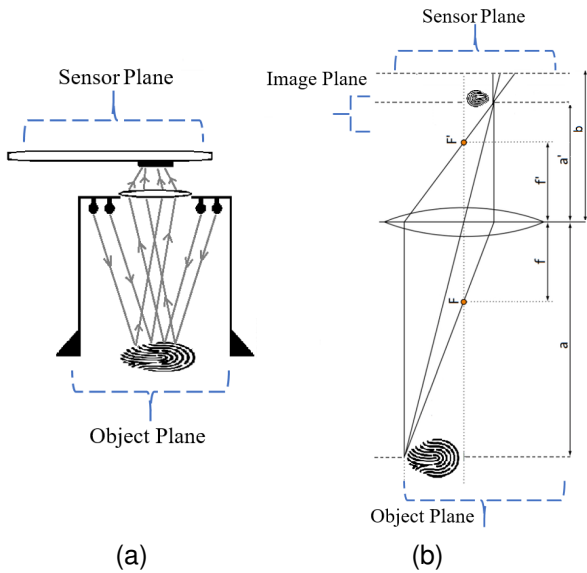
FIGURE 4. (a) Latent fingerprint acquisition apparatus, (b) positioning macro lens
