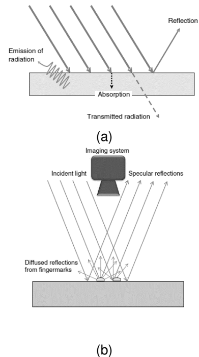
FIGURE 3. (a) Surface and light source interactions, and (b) the interaction of non-porous surfaces with light [47]
