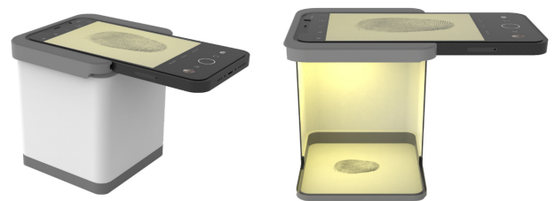
FIGURE 2. Latent fingerprint acquisition device apparatus
