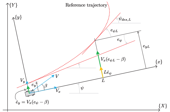
FIGURE 1. Look-ahead lateral dynamic model [33].
