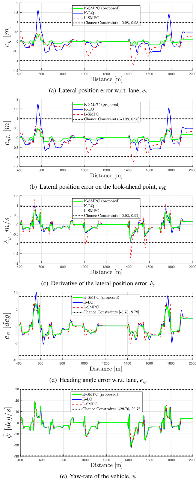
FIGURE 10. Control results of the system state.
