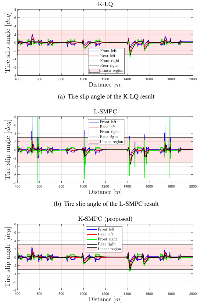
FIGURE 14. Results of the tire slip angle.
