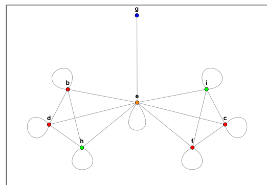
FIGURE 3. Images graph of the Dihedral group D_4 .
