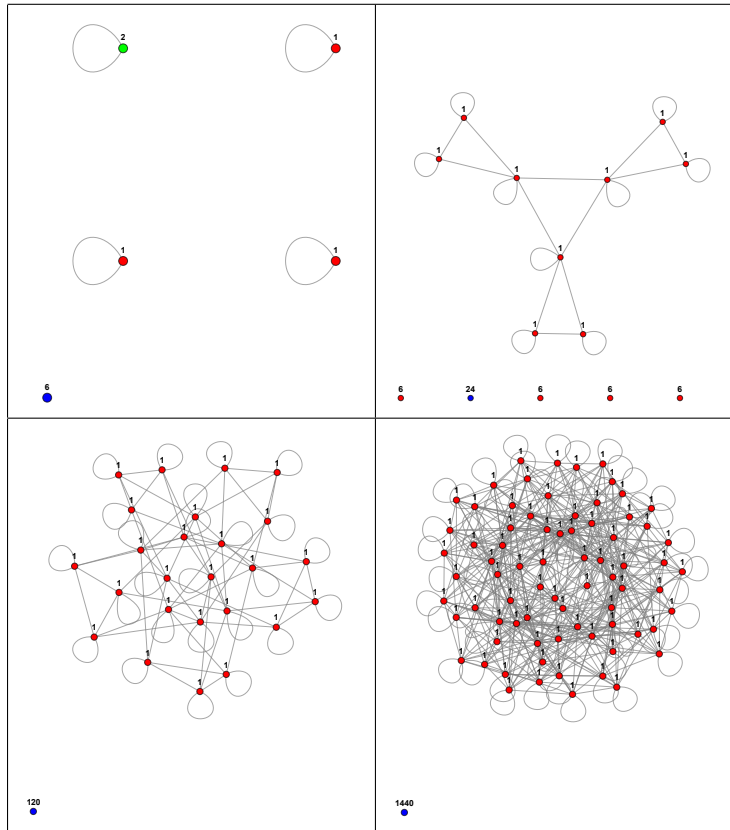
FIGURE 6. Images graphs of the symmetric groups S_3 to S_6 .
