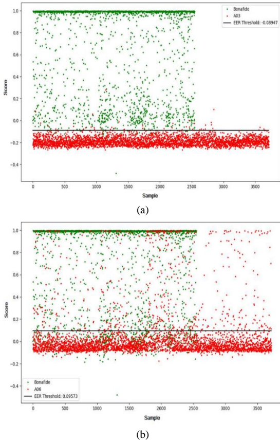
FIGURE 6. Score distribution of samples from A03 and A06 attack types using GLCM branch
