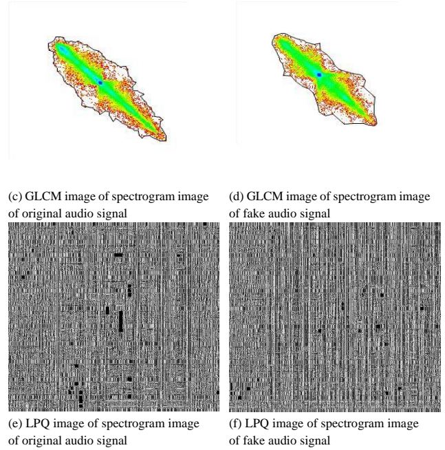
FIGURE 4. Three types of textural images for original and fake audios
