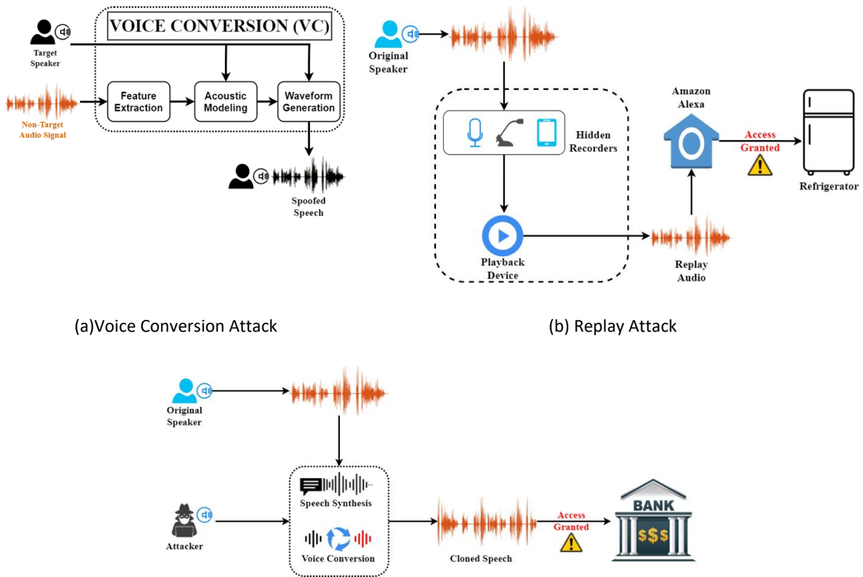
FIGURE 1. Various attack scenarios against ASV system (a) Voice conversion attack (b) Replay Attack (c) Synthetic speech attack
