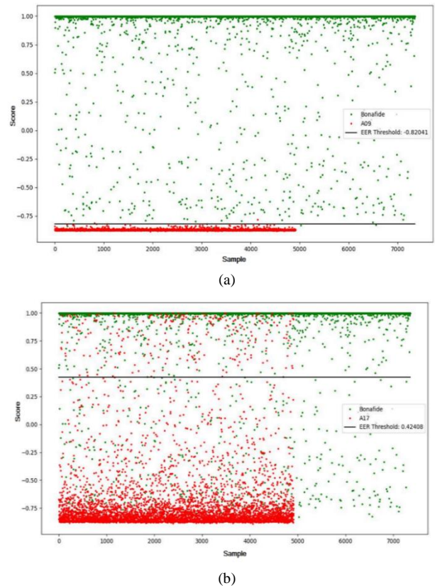
FIGURE 8. Score distribution of samples from A09 and A17 attack types using LBP branch
