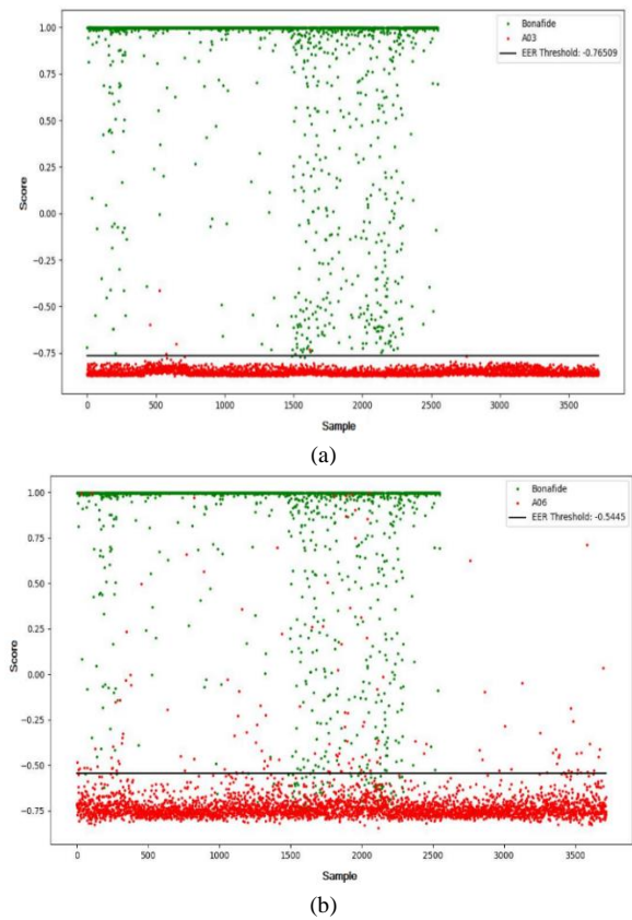
FIGURE 5. Score distribution of samples from A03 and A06 attack types using LBP branch
