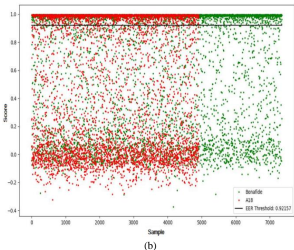
FIGURE 9. Score distribution of samples from A11 and A18 attack types using GLCM branch
