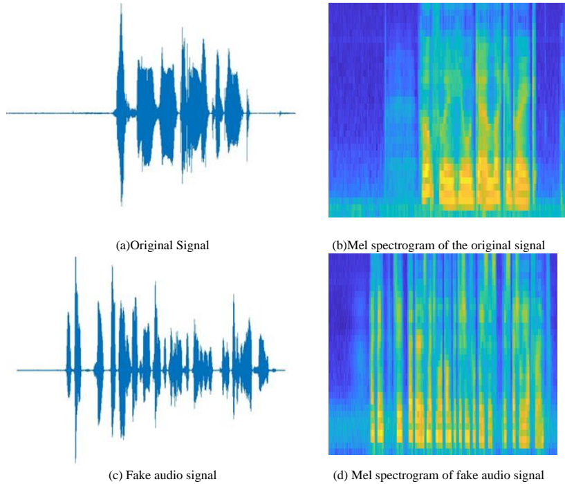
FIGURE 3. Mel spectrogram images of corresponding original and fake audio signals from ASVspoof 2019
