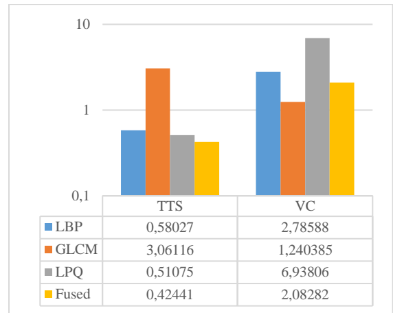
FIGURE 12. General performance of the fused system for Speech synthesis and Voice conversion attacks
