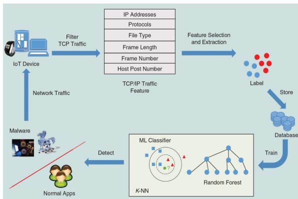
FIGURE 14. An Illustration of ML-Based Malware Detection using IOT
