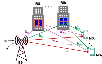
FIGURE 10. IRS-assisted DL communication system: multi-IRS and multi-user.
