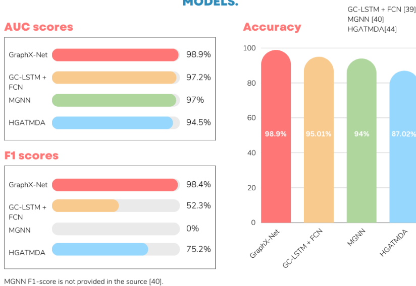
FIGURE 10. Detailed evaluation metrics breakdown of GraphX-Net and other GNNs models.
