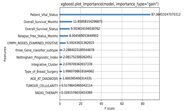
FIGURE 4. Visualizing Feature Importance with XGBoost Gain.
