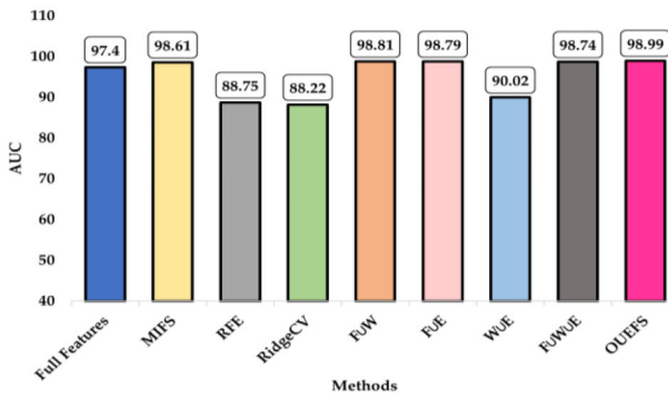
FIGURE 5. AUC comparison of all approaches.
