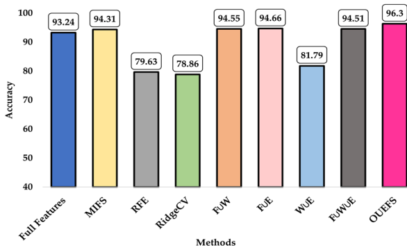
FIGURE 4. Accuracy comparison of all approaches.
