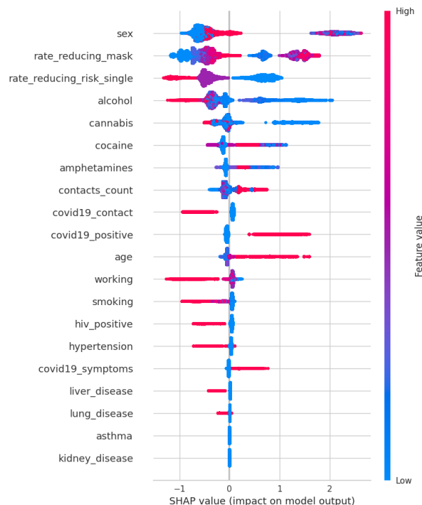
FIGURE 8. SHAP analysis.
