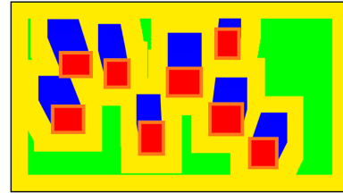
Fig. 4. Operative area, divided into available and occupied cells. Available cells are in green and correspond to the search space subdivided with the quadtree data structure. For the occupied cells, the red color is for the BBs, the orange color is for the BB borders, the yellow color is for the borders, and the blue color is for the occlusions.
