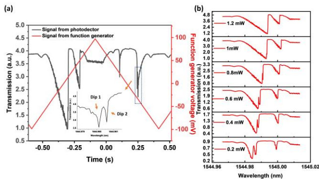
Fig. 8. (a) Dynamic response of the hollow core microbottle (98.9 \mu\text{m} ) at 1.2 mW pump laser power (black) and function generator signal (red), (b) transmission spectra of the hollow core microbottle at different pump laser power.
