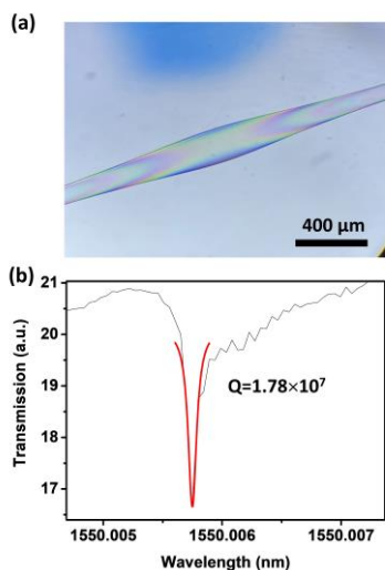
Fig. 1. (a) Microscopic image of the hollow-core microbottle, (b) transmission spectrum of the fiber taper coupled to the hollow-core microbottle and the Lorentzian fit of the resonance at 1550.0057 nm.
