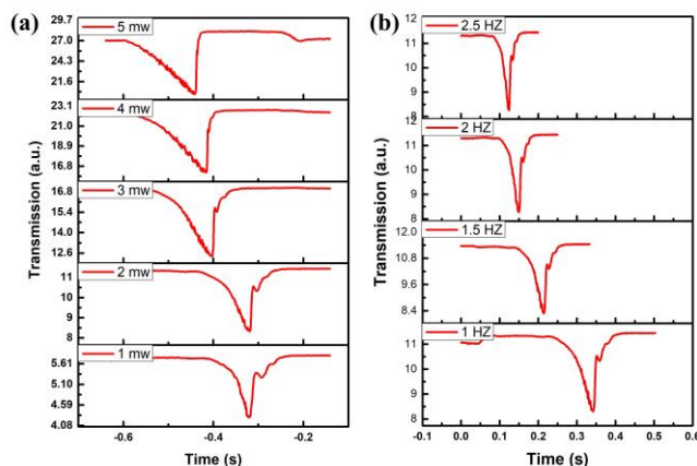
Fig. 4. Dynamic transmission responses of the hollow core microbottle at (a) different pump powers and constant scanning frequency of 1 Hz, (b) different laser scanning frequencies and fixed pump laser power of 2 mW.
