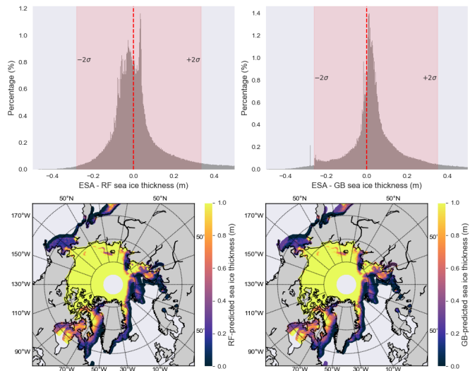
Fig. 4. a) Upper: Histograms of the difference between the ESA’s official sea ice thickness product and the predicted sea ice thickness using the Random Forest and the Gradient Boosting algorithms, respectively, for January 2022. b) Lower: Arctic sea ice thickness maps generated with the Random Forest and Gradient Boosting algorithms, respectively, for 31st January 2022.
