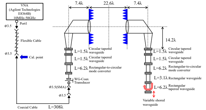
Fig. 5 Measurement system of simplified model.
