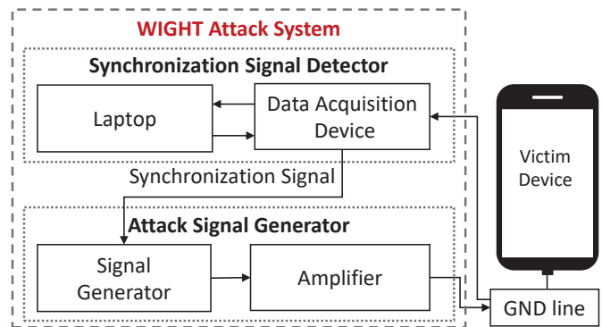
Fig. 17. An illustration of WIGHT attack system.
