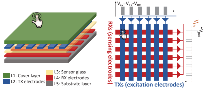
(a) Overview of touchscreen. (b) Top view of electrodes.
