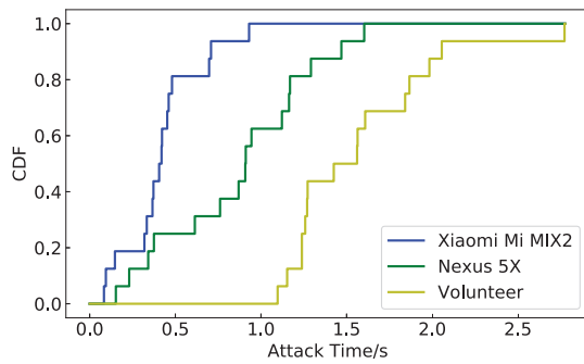
Fig. 22. The CDF plots about the response time of WIGHT attack and volunteers. The average response time of WIGHT on Xiaomi Mi MIX2 is 0.420 s and on LG Nexus 5X is 0.872 s, on volunteers is 1.523 s.
