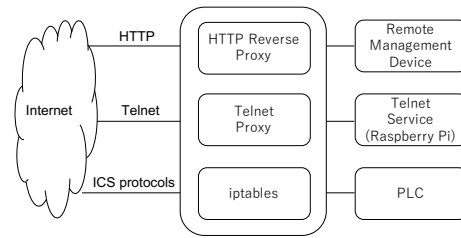
Fig. 5. Honeypot architecture
