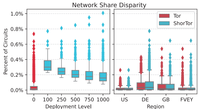
Fig. 10: Fraction of circuits seen by relays in Tor vs. ShorTor. Left side considers incremental deployment (Section IV-C3). As more relays begin to support ShorTor (x-axis), the average network share goes down, though some outliers see more traffic. Right side looks at regional network share, or the fraction of circuits seen by relays in different regions.
