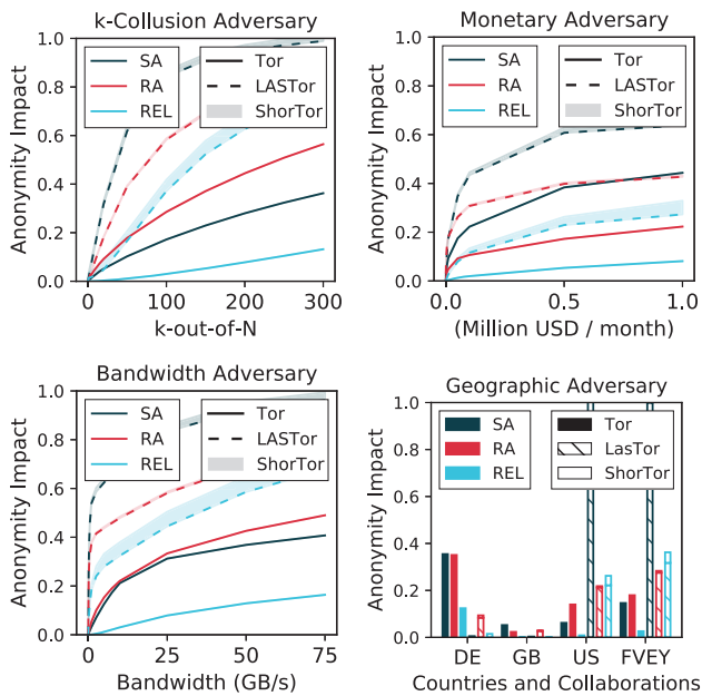
Fig. 9: Anonymity impact of ShorTor, compared with baseline Tor (client-independent) and LASTor (dependent on client location) path selection. Each plot shows sender (SA), recipient (RA), and relationship (REL) anonymity (Definition V.1) for a different adversarial relay corruption strategy. Shaded region represents the difference in the MATOR-computed anonymity bounds with and without ShorTor. “FVEY” refers to “Five Eyes” intelligence alliance member countries. Under ANoA, ShorTor affects all anonymity notions for LASTor, though not baseline Tor. Extended plots provided in Appendix A.
