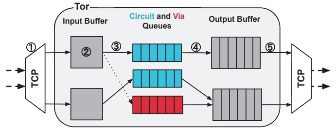
Fig. 5: Tor relay with circuit and via traffic (queuing architecture unmodified from baseline Tor). ① Via and circuit traffic are multiplexed on a TCP connection entering the Tor relay. ② The TLS layer is decrypted and circuit cells are onion encrypted/decrypted. ③ Circuit and via cells are sent to their individual queues. ④ Cells are scheduled for release to the output buffer based on priority order. ⑤ The contents of the output buffer are encrypted using TLS, then sent to the kernel for transit over a TCP connection to the next hop.
