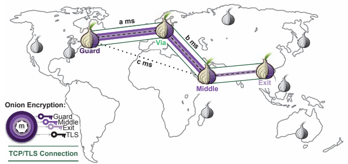
Fig. 3: A Tor circuit routing using a via relay between the guard and middle. A via relay will be used when the latency over the via ( a+b ms) is less than that of the direct connection ( c ms). The via does not participate in onion routing. For clarity, and because ShorTor only operates between Tor relays, the client and server are not shown.
