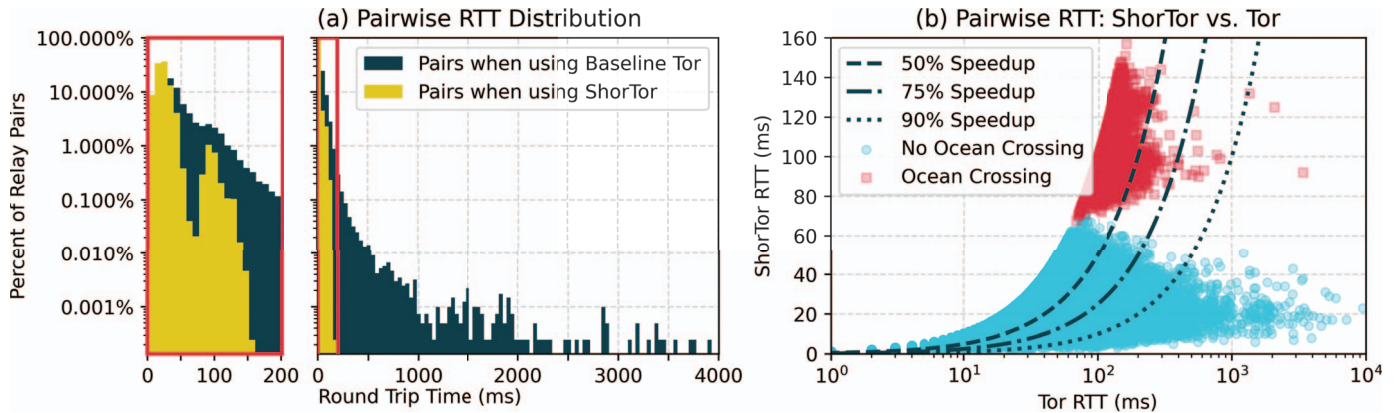
Fig. 6: (a) Left: Round-trip times (RTTs) measured between Tor relays vs. RTTs of those same pairs when using ShorTor as a percentage of all 406,074 pairs. We show an expanded view of the first 200 ms on the left. For readability, this figure omits 10 pairs with RTTs between 4,019 ms and 9,415 ms. (b) Right: Relative latency of each relay pair when routing via ShorTor vs. the default route. 25.4 % of pairs have a latency reduction of at least 50 %, 9.4 % at least 75 %, and 1.2 % at least 90 %.
