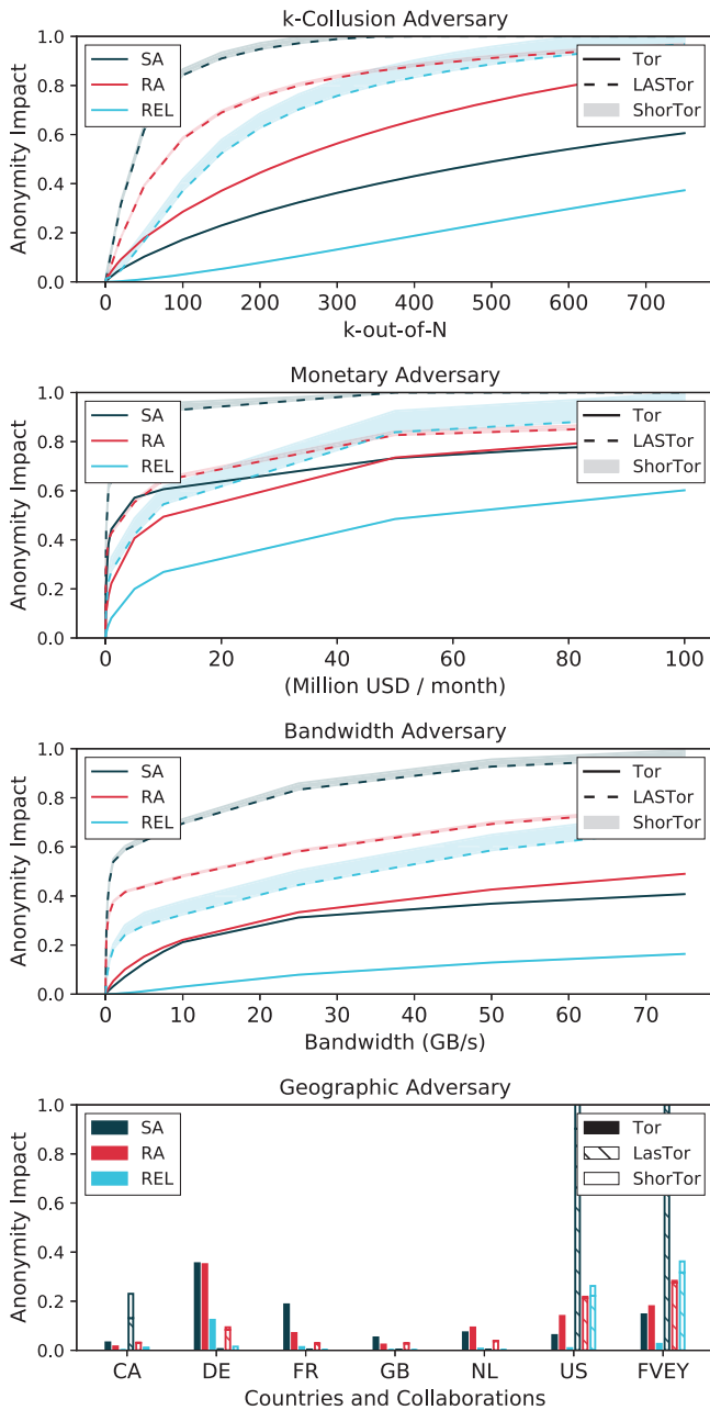
Fig. 11: Extended experiments for the anonymity impact of ShorTor. Anonymity impact of ShorTor, compared with baseline Tor (client-independent) and LASTor (dependent on client location) path selection. Each plot shows sender (SA), recipient (RA), and relationship (REL) anonymity (Definition V.1) for a different adversarial relay corruption strategy. Shaded region represents the difference in the MATOR-computed anonymity bounds with and without ShorTor. “FVEY” refers to “Five Eyes” intelligence alliance member countries. Under ANoA, ShorTor affects all anonymity notions for LASTor, though not baseline Tor.
