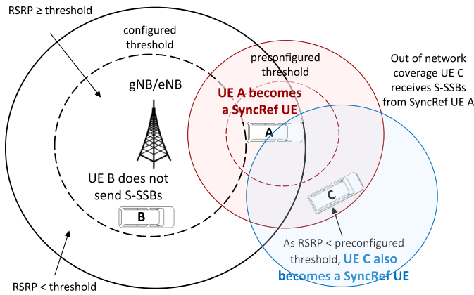
Fig. 14. Triggering of S-SSB transmissions when RSRP of synchronization reference is lower than a threshold, where the threshold is (pre-)configured.
