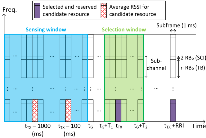
Fig. 2. LTE V2X channelization and illustration of mode 4 sensing-based SPS scheduling (illustrative example when T=100 ms).
