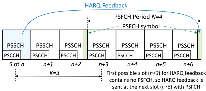
Fig. 10. PSSCH-to-HARQ feedback timing based on at least K = 3 slots. For simplicity, the figure depicts only one sub-channel within the resource pool. We also omit the detailed structure of a PSCCH/PSSCH slot with or without PSFCH including PSSCH DMRS, AGC symbols and guard symbols.
