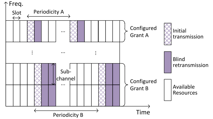
Fig. 23. Multiple active UL configured grants for NR V2N communications.
