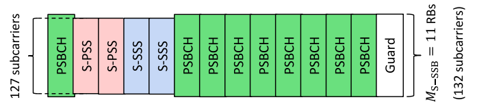
Fig. 7. S-SSB including PSBCH, S-PSS and S-SSS (for normal CP).
