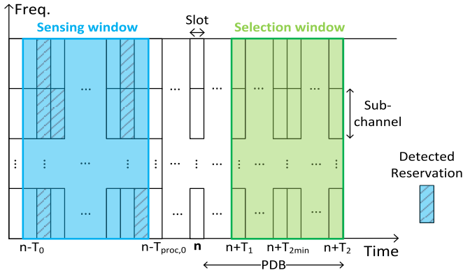
Fig. 18. Sensing and selection windows of NR V2X SL mode 2 when T_2 = \text{PDB} .
