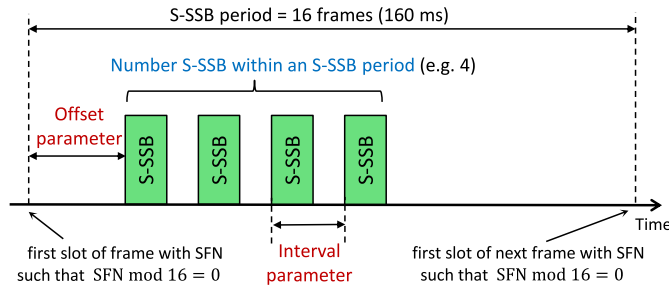
Fig. 8. Multiple S-SSB transmissions within an S-SSB period.
