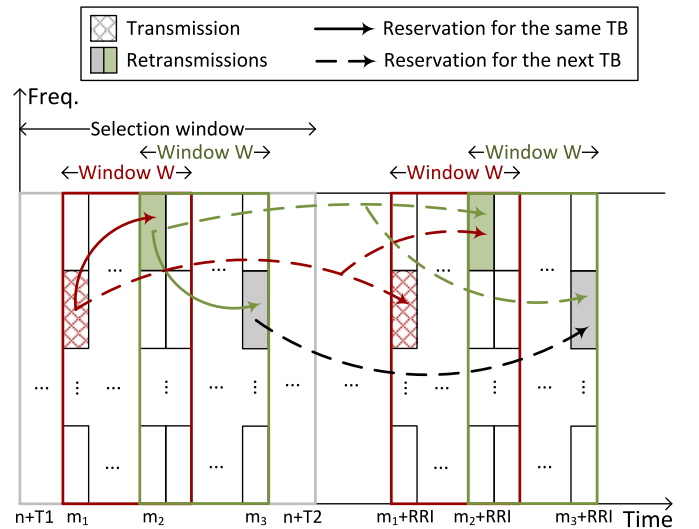
Fig. 19. Resource reservation for the retransmissions of the same TB and for the transmission and retransmissions of the next TB in NR V2X mode 2 (illustrative example when N = 3 , \max(N_{SCI}) = 3 and RRI (in number of slots)). The transmission of the TB at m_1 does not announce the reservation of the retransmission at m_3 because it is outside of the window W . This reservation for the second retransmission is announced by the first retransmission at m_2 .
