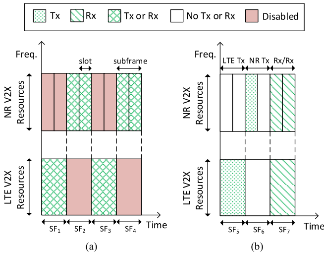
Fig. 26. TDM solutions for the coordination between RATs. (a) Long-term. (b) Short-term.
