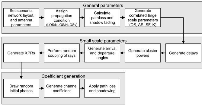
Fig. 28. Channel generation procedure for V2V SL (adapted from [104]).
