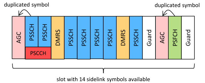
Fig. 6. Example of a PSCCH/PSSCH slot with a PSFCH, 2 PSCCH, 9 PSSCH including 2 PSSCH DMRS symbols (for normal CP).
