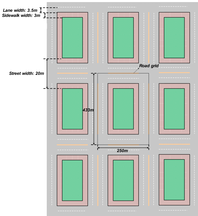
Fig. 31. Road configuration for urban grid (adapted from [103]).
