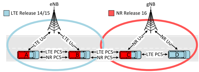
Fig. 25. Coexistence between NR V2X and LTE V2X.
