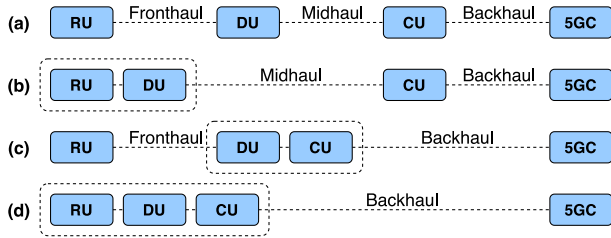
Fig. 12. 5G Fronthaul, Midhaul and Backhaul Combinations [124].
