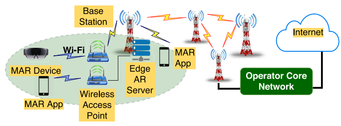
Fig. 6. Edge based System Architecture for a MAR System.
