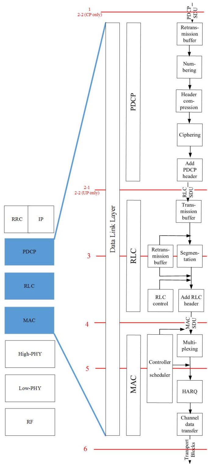
Fig. 4. Functional splits in the Data Link layer illustrating the exact location of the functional splits proposed by 3GPP [10] marked by red lines. Split 2-2 is a special case having one split for the Control Plane (CP) and another one for the User Plane (UP).
