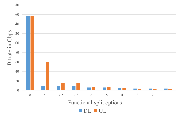
Fig. 6. Fronthaul bitrates, as per 3GPP [9] UL and DL for each functional split.
