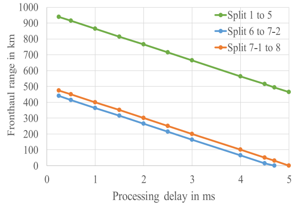
Fig. 9. Length of fronthaul depending on processing delay.
