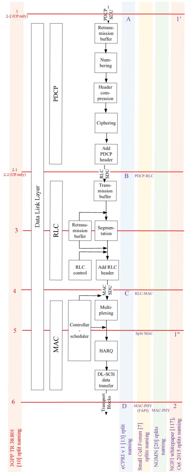
Fig. 8. Functional splits in the Data Link Layer illustrating the differences in the splits investigated by different standardization organizations.
