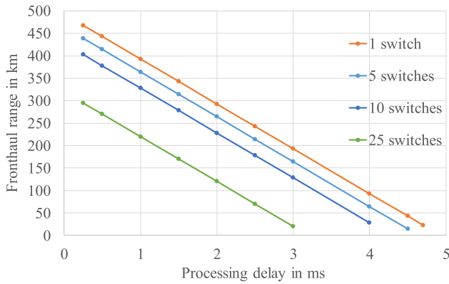
Fig. 10. Length of fronthaul depending on processing delay illustrated for splits 6 to 7-2 having the HARQ process in the CU. The figure shows how the fronthaul length also depends on how many switches the data needs to be processed through as each switch adds delay.
