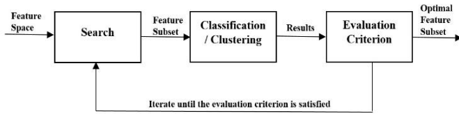
Fig. 2. Wrapper Method Topology.
