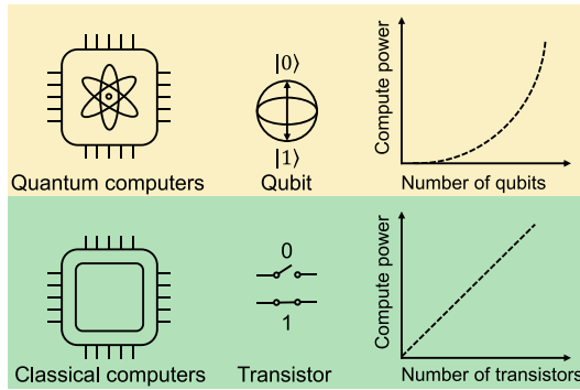
Fig. 1. Comparison of computational power between quantum computers and classical computers. The symbol ‘ |\cdot\rangle ’ is the notation for quantum states, which will be elaborated on in further detail in Section III-A1.
