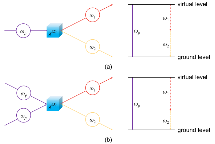
Fig. 15. Schematic portrayal and energy-level diagram of (a) spontaneous parametric down-conversion and (b) spontaneous four-wave mixing.
