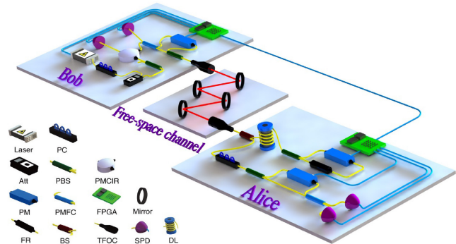
(d) Free-space QSDC system [96]. Reprinted with permission from Ref. [96] © The Optical Society.
