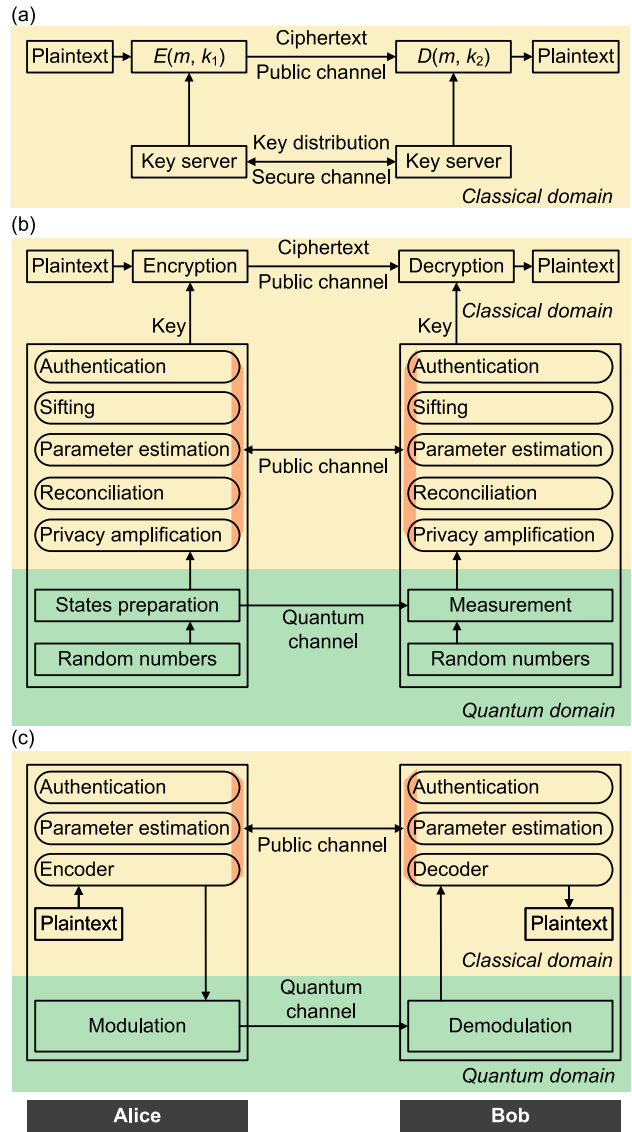
Fig. 3. Different models of communication systems. (a) classical cryptosystem. (b) QKD system. Key agreement is carried out by QKD, and information is transmitted via classical communication, the same as in (a). (c) QSDC system. No key distribution, no key management and no ciphertext are required in QSDC.
