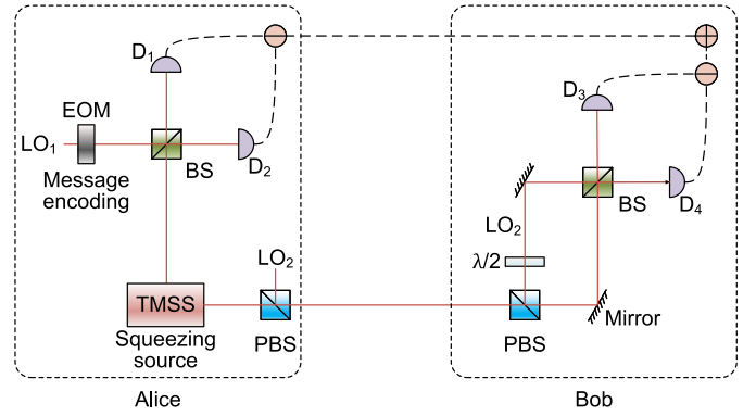
Fig. 25. Schematic of the CV DSQC protocol using two-mode squeezed states. LO: local oscillator, EOM: electro-optical modulator, BS: beam splitter, TMSS: two-mode squeezed state, PBS: polarizing beam splitter, D: photodetector, \lambda/2 : half wave plate.
