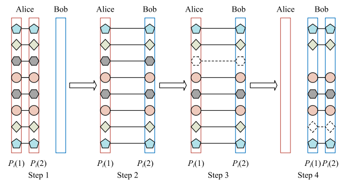
Fig. 20. Schematic illustration of the high-capacity QSDC protocol. Two symbols linked with a line are in a Bell-state. The pentagons, the rhombuses, the hexagons, and the circles represent the Bell state |\phi^+\rangle_{AB} , |\phi^-\rangle_{AB} , |\psi^+\rangle_{AB} , and |\psi^-\rangle_{AB} , respectively. The blank dashed symbols represent the state after Alice and Bob complete eavesdropping detection.
