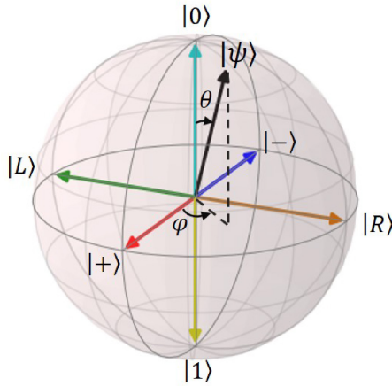
Fig. 7. Visualization of qubit states in the Bloch sphere.
