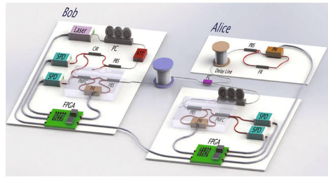
(b) QSDC system over 1.5 km fiber channel [70]. Reprinted with permission from Ref. [70] © Springer Nature.
