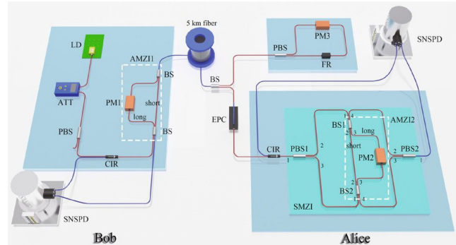
(f) QSDC without active polarization compensation [103]. Reprinted with permission from Ref. [103] © Springer Nature.
