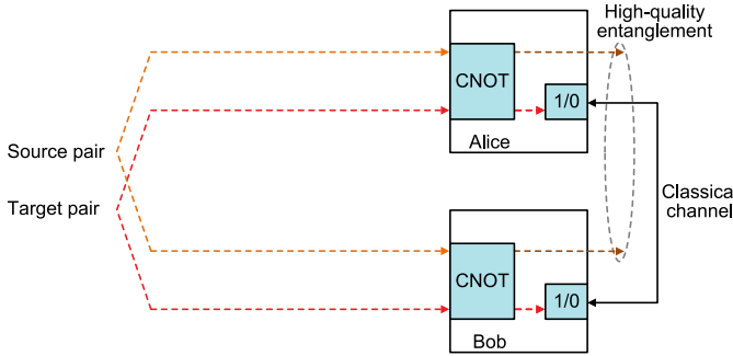
Fig. 13. The Scheme of entanglement purification by Bennett et al. [185]. CNOT: Controlled-NOT.
