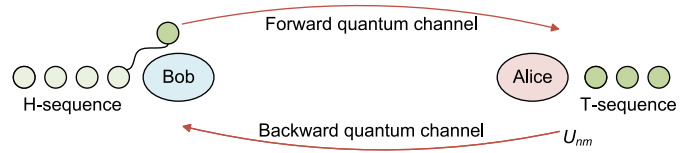
Fig. 23. Scheme showing principles involved in the high-dimension two-step QSDC of [71]. The connected circles represent an EPR pair. The bottle green circle is the EPR partner particle that belongs to what we refer to as T-sequence, while the light green one belongs to the H-sequence. U_{nm} is the unitary transformation used for encoding.
