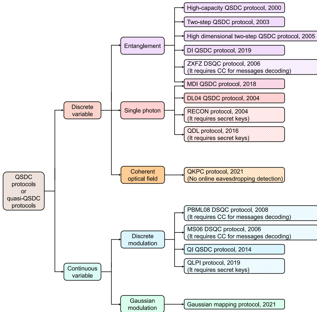
Fig. 26. The evolution of the QSDC protocols or quasi-QSDC protocols. This diagram is an extension based on [49], which includes the following protocols: High-capacity QSDC protocol [42], Two-step QSDC protocol [63], High dimensional two-step QSDC protocol [71], Device independent (DI) QSDC protocol [92], Zhu-Xia-Fan-Zhang (ZXFZ) DSQC protocol [128], Measurement-device-independent (MDI) QSDC protocol [88], Deng-Long 2004 (DL04) QSDC protocol [64], Repeatable classical one-time-pad (RECON) protocol [384], Quantum data locking (QDL) protocol [87], Quantum keyless private communication (QKPC) protocol [99], Pirandola-Braunstein-Mancini-Lloyd 2008 (PBML08) protocol [77], Marino-Stroud 2006 (MS06) protocol [129], Quantum illumination (QI) QSDC protocol [84], Quantum low probability of intercept (QLPI) protocol [91], and Gaussian mapping protocol [307]. CC: classical communication. The protocol marked with grid-patterned color is referred to as quasi-QSDC.
