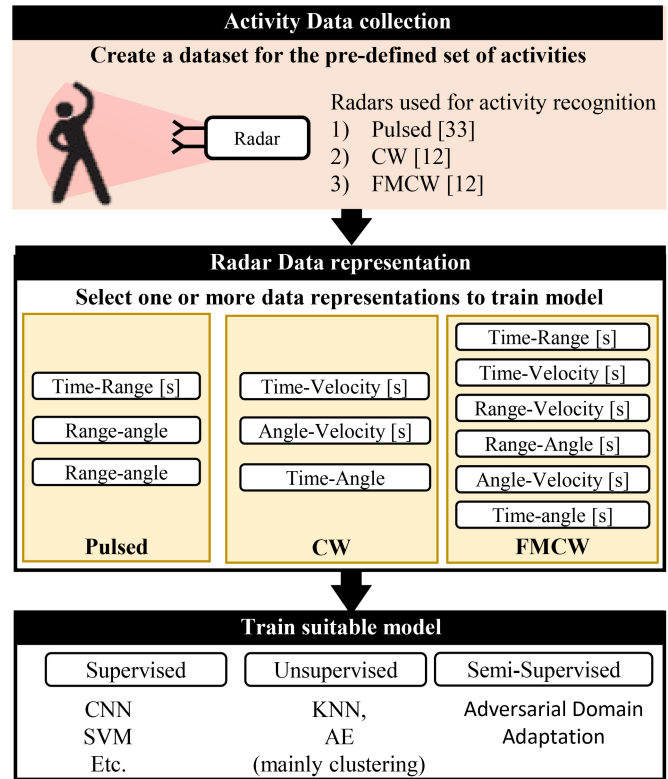
Fig. 9. Radar based activity recognition framework.
