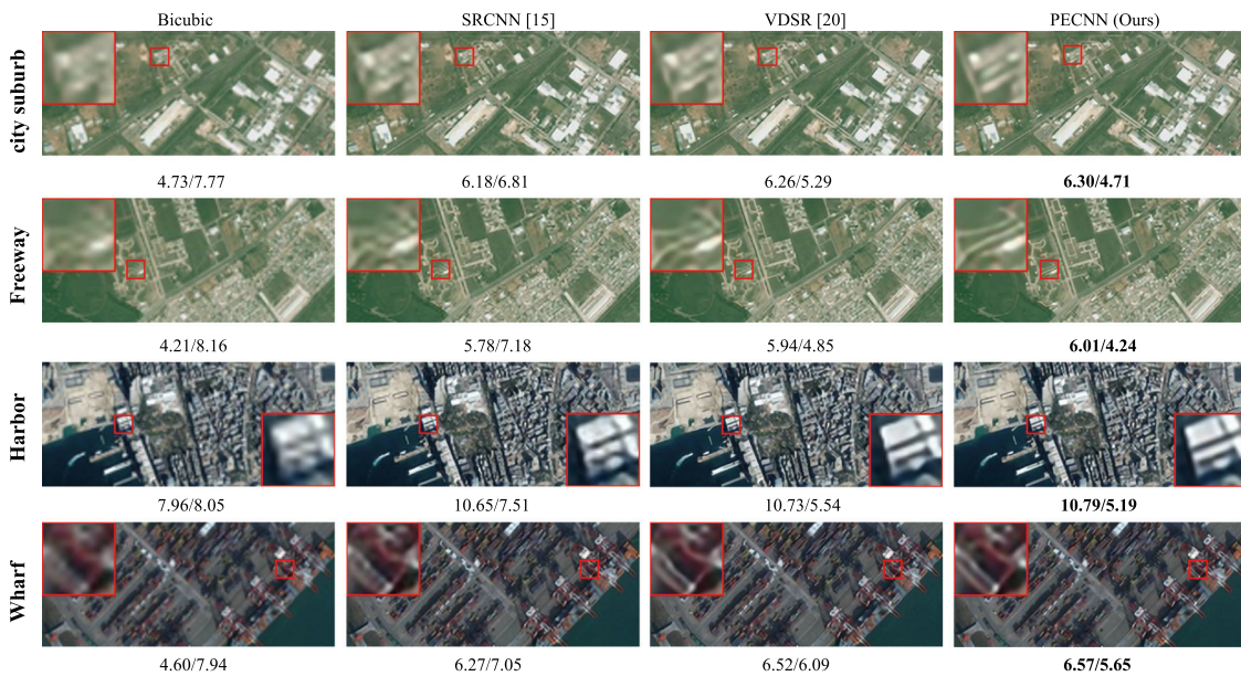
Comparison results on Jilin-1 satellite imagery with scaling factor \times 3 . The bold indicates the best performance (AG/NIQE). For more information, see "A Progressively Enhanced Network for Video Satellite Imagery Superresolution" by Jiang, et al. , p. 1633.
