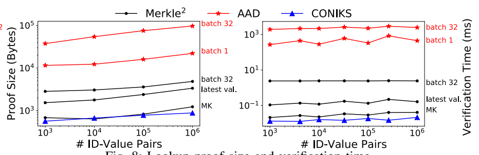
Fig. 8: Lookup proof size and verification time.
