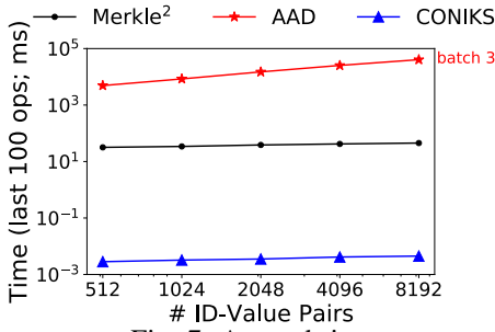
Fig. 7: Append time.
