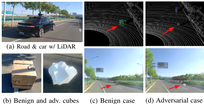
Figure 8: Physical-world experiment settings and evaluation results for LiDAR-side physical-world attack realizability. We use a Velodyne HDL-64E LiDAR mounted on a real vehicle. The adversarial cube is 3D-printed at 1:1 scale.
