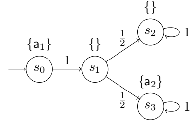
Fig. 2. HyperPCTL* example on DTMC \mathcal{M} .
