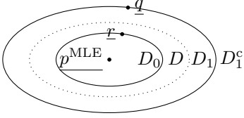
Fig. 7. Given the test region D , we assume there exists an indifference region formed by D_1 \setminus D_0 . If p^{\text{MLE}} from (35) satisfies p^{\text{MLE}} \in D_0 , then we find \underline{r} \in D_0 by (41) and \underline{q} \in D_1^c by (37).
