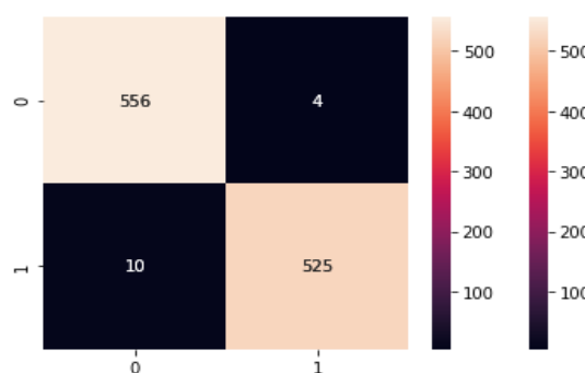
Fig.5 Confusion Matrix
