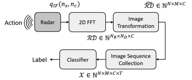
Fig. 1. Block diagram of the action elaboration.
