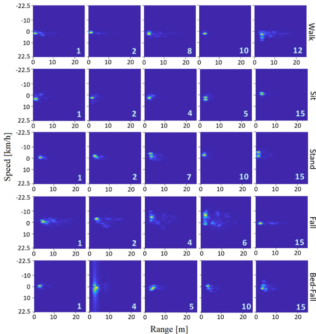
Fig. 7. Example of range-Doppler maps for the five actions.
