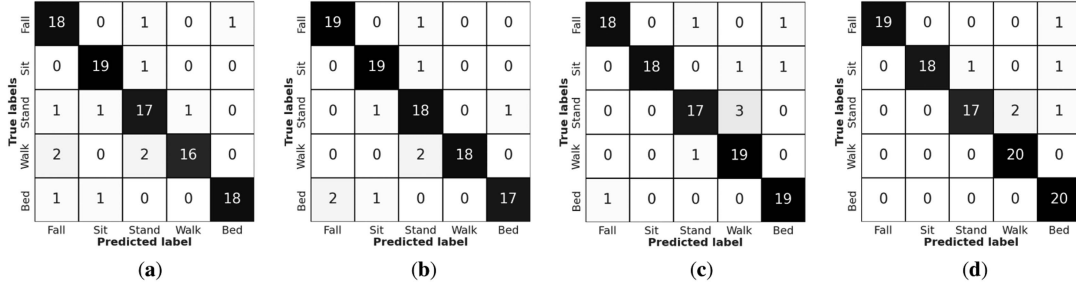
Fig. 13. Confusion matrixes of DNN2 and DNN3 computed on the new dataset with no transformation and in grayscale. (a) DNN2 tested on \mathcal{T}_{\text{Orig}} . (b) DNN2 tested on \mathcal{T}_{\text{Gray}} . (c) DNN3 tested on \mathcal{T}_{\text{Orig}} . (d) DNN3 tested on \mathcal{T}_{\text{Gray}} .
