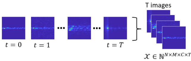
Fig. 3. Example of a 4-D tensor representing an action.
