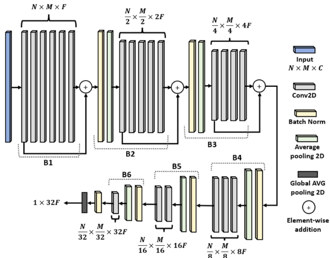
Fig. 5. CNN2 architecture.
