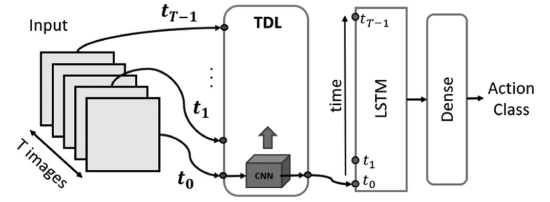
Fig. 4. Proposed DNN.
