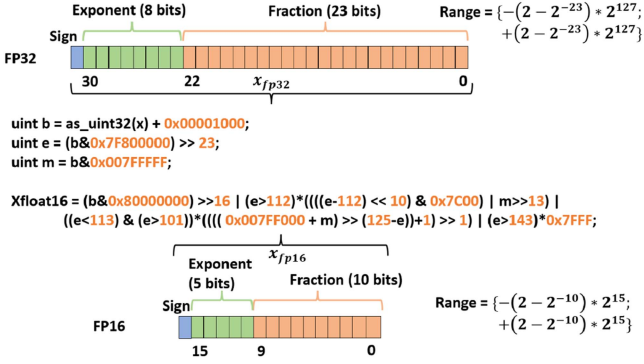
Fig. 8. Quantization from FP32 to FP16.
