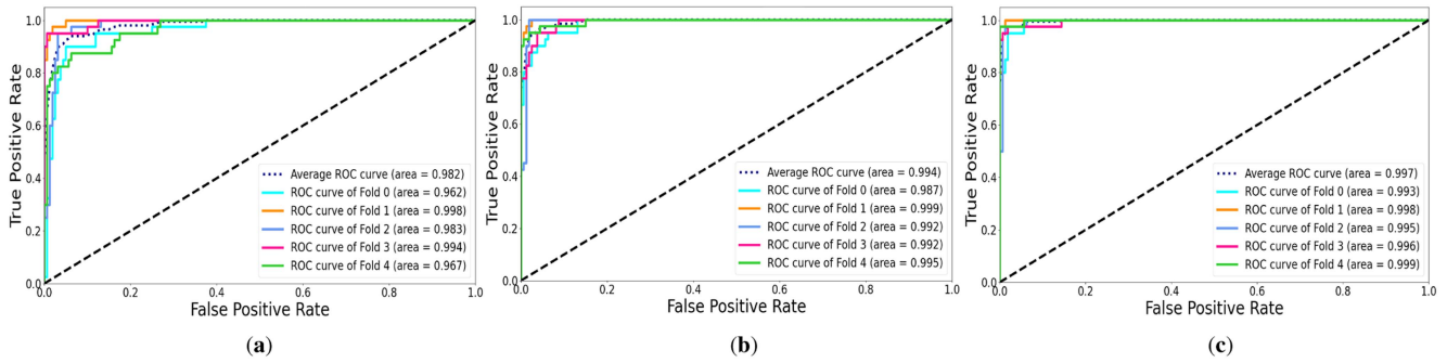
Fig. 10. ROC and AUC computed over the folds of the best performing models. (a) DNN1 trained on \mathcal{D}_{\text{Canny}} . (b) DNN2 trained on \mathcal{D}_{\text{Gray}} . (c) DNN3 trained on \mathcal{D}_{\text{Gray}} .
