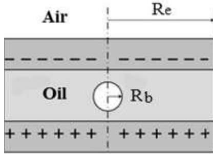
Figure 1. The void inside of plane capacitor. Here it is shown charges distribution before partial discharge.
