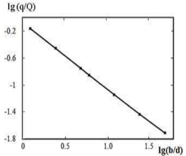
Figure 4. “Apparent” charge to true charge ratio for different bubble radius. Here d = 2R_b .
