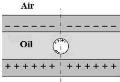
Figure 2. Over-simplified charge distribution after PD.
