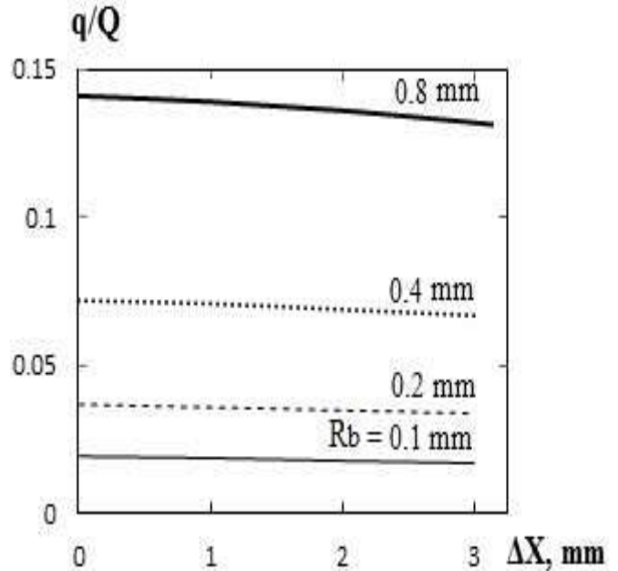
Figure 5. “The apparent” charge to the true charge ratio for bubbles with different radius on the shift distance \Delta X
