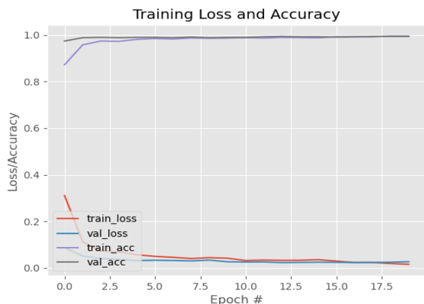
Fig. 4. Training Model accuracy and loss curves
