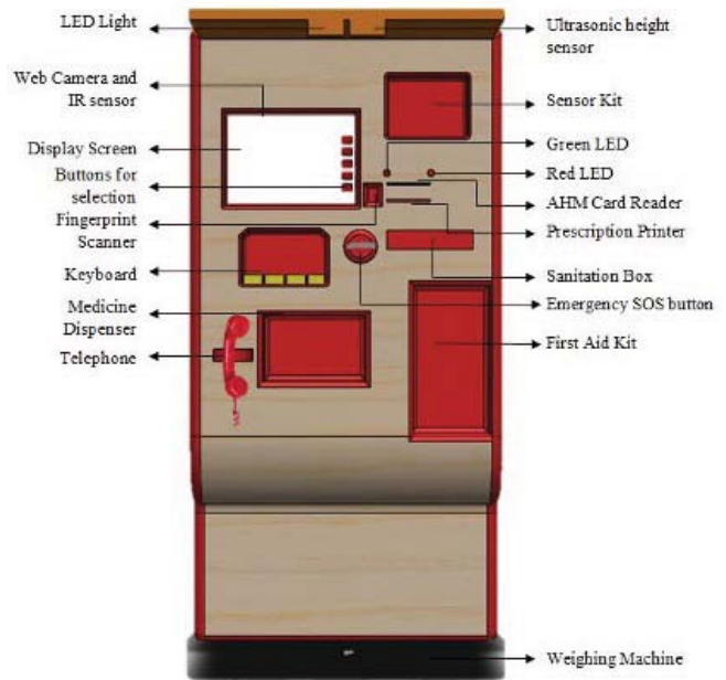
Fig. 4. Front view of the Automatic Health Machine
