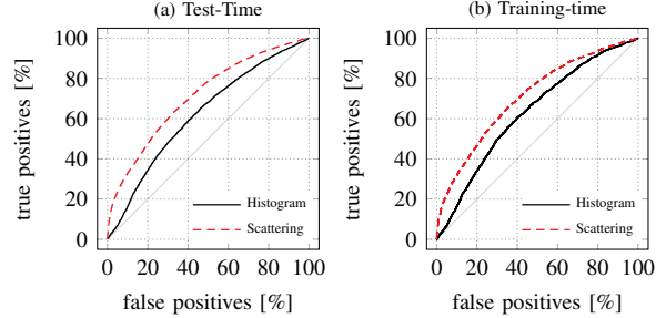
Fig. 7. Defenses against backdoor attacks: ROC curves of histogram-based and color scattering-based method. Both do not reliably detect image-scaling attacks that hide backdoors.
