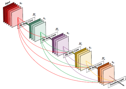
Fig. 4. DenseNet Architecture [17].
