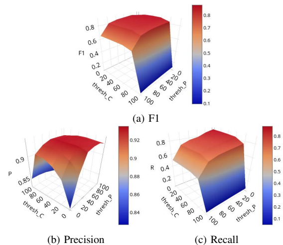
Figure 11: Accuracy sensitivity analysis at varying detection threshold values.
