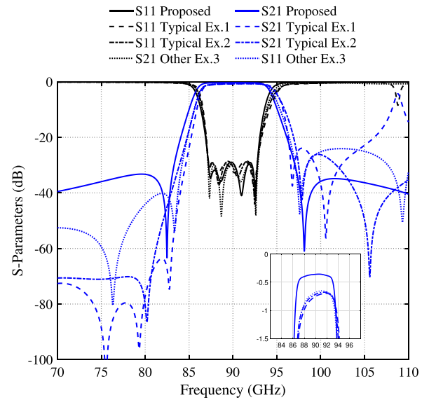
FIGURE 21. Simulated S-parameters of fourth-order single- and dual-TM-mode filters with FBW = 6.2\% . The proposed dual-mode filter takes the form of Fig. 20(a), dual-mode examples (Ex.1 and Ex.2) take the form of Fig. 20(b), and the single-mode example (Ex.3) takes the form of Fig. 20(c). (equivalent conductivity of all filters is taken as 5.9 \times 10^6 S/m).
