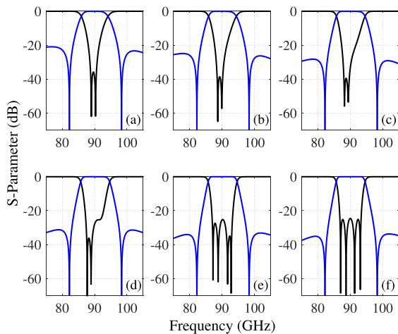
FIGURE 12. Evolution of the simulated S-parameter response for the proposed dual-mode filter specified in Fig. 6 while varying the resonant slot-iris thickness value ( I_z ). For images (a) through (f), I_z = 0.1 mm, 0.275 mm, 0.45 mm, 0.625 mm, 0.8 mm, and 0.868 mm respectively. (re-optimized dimensions not shown).
