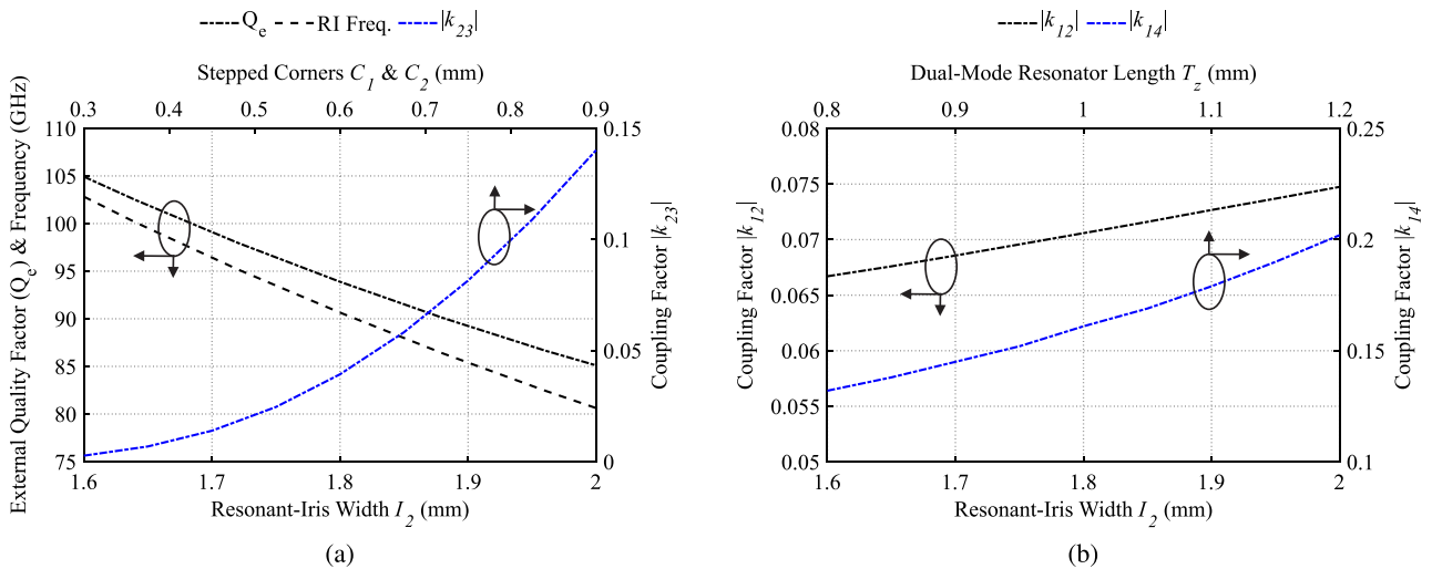
FIGURE 11. Effects of parameter variation on the external quality factor, coupling values and resonant-iris frequency for the filter specified in Fig. 6. (a) External quality factor, resonant-iris frequency, and coupling factor k_{23} 's dependence on resonant-iris width I_2 and stepped corner sizes C_1 and C_2 , and (b) Coupling factor k_{12} and k_{14} 's dependence on resonant-iris width I_2 and the dual-mode resonator length T_z .
