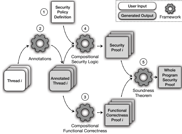
Figure 2: Proving a program secure in VERONICA.
