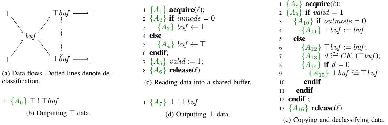
Figure 1: Co-operative Use of a Shared Buffer. Green \{A_i\} are functional correctness annotations (whose contents we omit).
