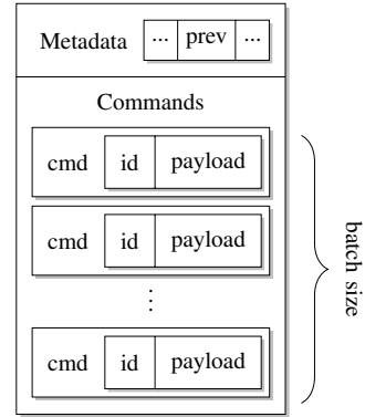
Fig. 6: Structure of a block in the implementation.
