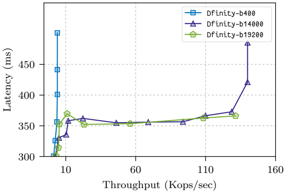
Fig. 9: Throughput vs. latency of Sync HotStuff at varying batch sizes at \Delta = 50 ms and f = 1 for Dfinitiy [13].
