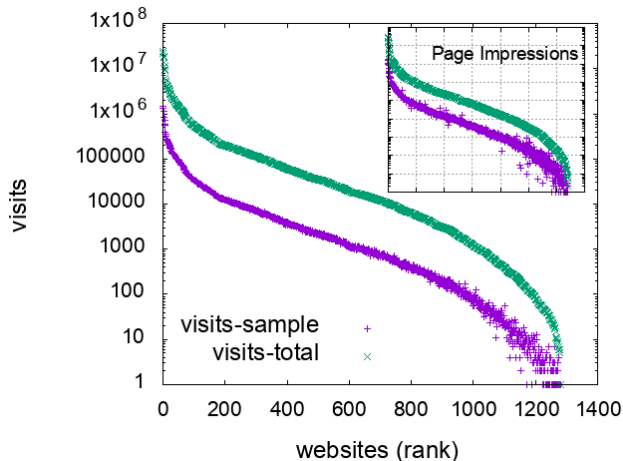
Fig. 1. Distribution of visits: sample vs entire dataset (PIs in inset). Websites are ranked by the number of visits in the original dataset. The sample distribution largely follows the original distribution, meaning websites are represented proportionally in the sample.
