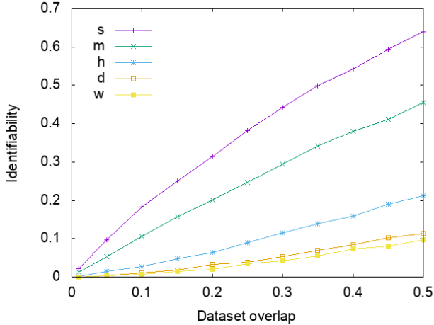
Fig. 8. Dataset enrichment via acquiring a dataset: We measure the identifiability of the acquired dataset given an overlap between the datasets. Configuration: ./-/-/site/∞
