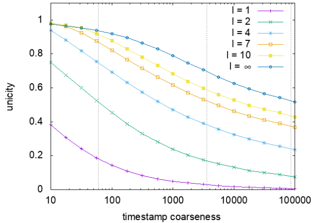
Fig. 3. Click trace unicity, trace length limited to l . Configuration: x/loc/code/site/-.
