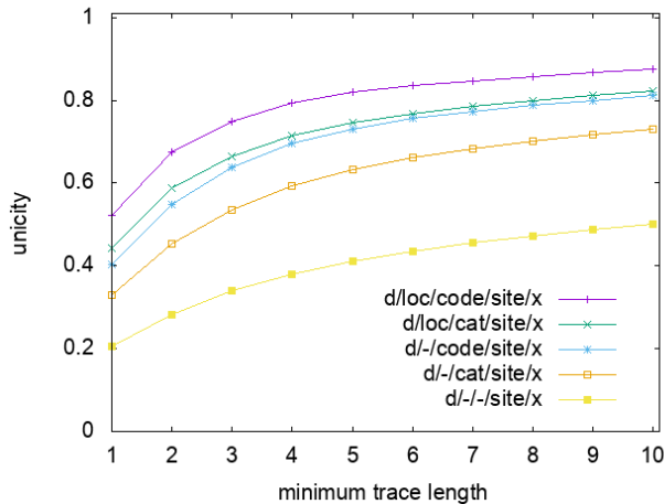
Fig. 4. Click trace unicity with minimum length, timestamps coarsened to the day.
