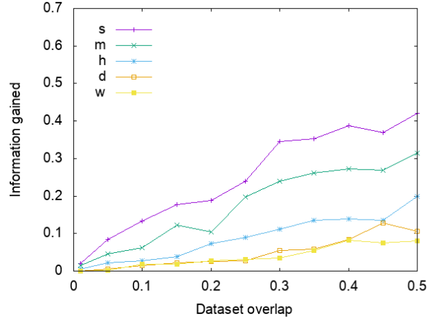
Fig. 9. Dataset enrichment via acquiring a dataset: We measure the information gain, meaning the amount of information in identified click traces not previously known, given the overlap between datasets. Configuration: ./-/-/site/∞
