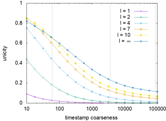
Fig. 6. The “Matomo (Piwik) case”, local unicity at max length l . Configuration: x/-/cat/-/.
