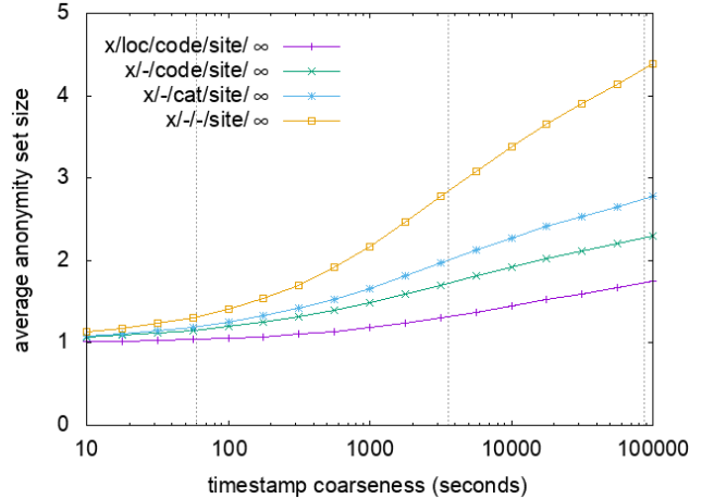
Fig. 7. Average anonymity set size within the original dataset.
