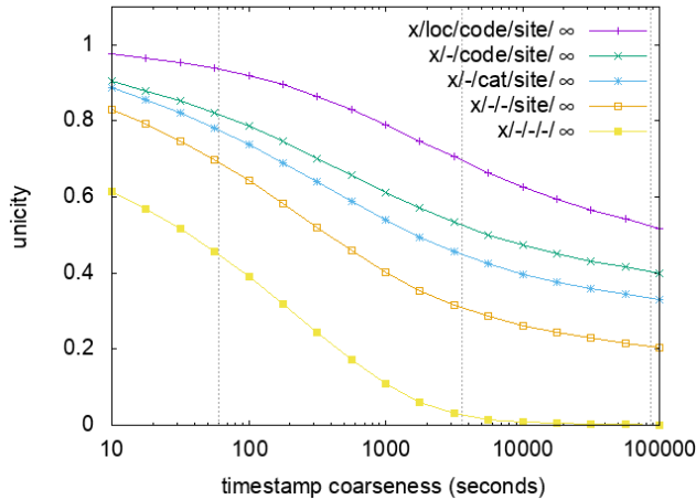
Fig. 2. Click trace unicity over coarsened time.
