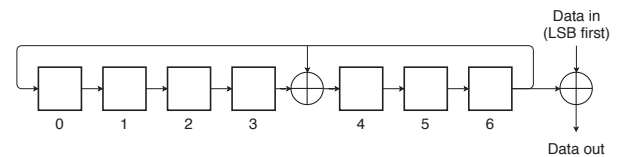
Fig. 3: LFSR used for frame (de-)whitening. Bits 0 to 5 are initialized with bits clk_{1-6} of the master’s clock; bit 6 is always initialized with 1.
