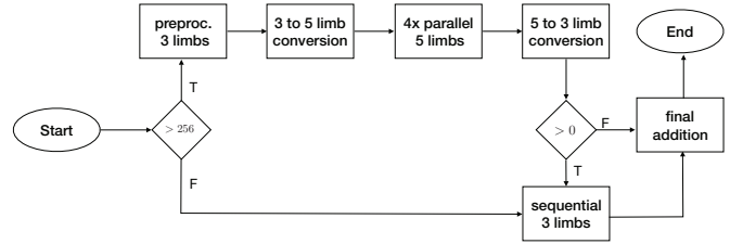
Figure 3: Structure the optimized Poly1305 implementation.
