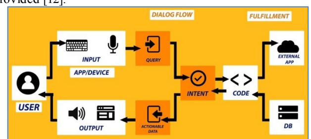
Fig 1. The Architecture of the Conversational Bot
