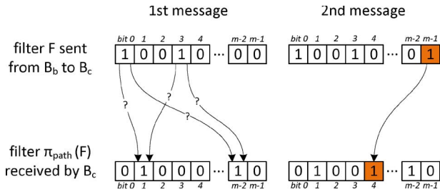
Fig. 5. Solving (partially) the composite permutation between two bots by turning 0-bits to 1-bits.
