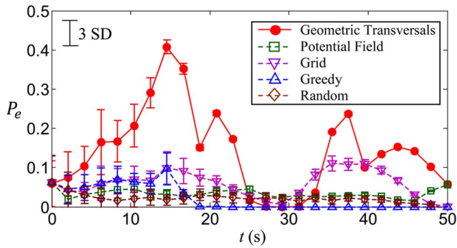
Fig. 8. Probability of detection averaged over 100 initial conditions for n = 20 , r_i = 5 (m), and the target motion model in Table I.
