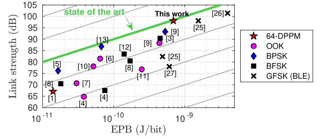
Fig. 18. Link strengths of the works included in Table III versus EPBs.
