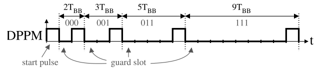
Fig. 2. Example of an 8-DPPM data packet. [1, Fig. 2].
