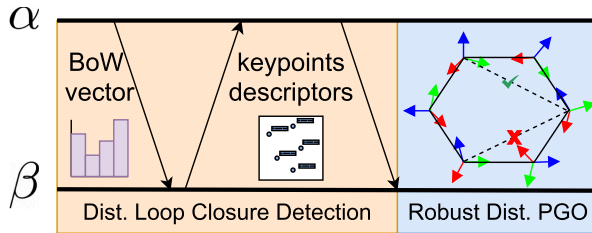
Fig. 3. Communication protocol and data flow between a pair of robots.
