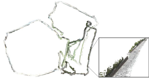
Fig. 15. Stata experiment . Optimized mesh produced by Kimera-Multi corresponding to trajectory estimate shown in Fig. 14(c).
