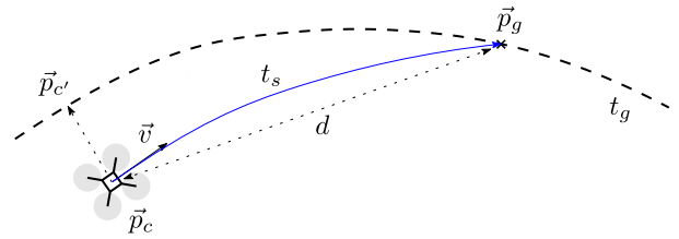
Fig. 2. Pose \vec{p}_c of the quadrotor is projected on the global trajectory t_g to find the point \vec{p}_{c'} . The point at distance d from the current quadrotor position \vec{p}_c , which belongs to t_g in the forward direction with respect to \vec{p}_{c'} , defines the desired goal position \vec{p}_g . To push the quadrotor toward the reference trajectory t_g , a short trajectory segment t_s is planned and tracked in a receding horizon fashion.
