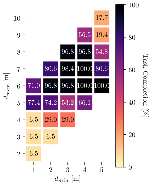
Fig. 7. Sensitivity analysis of planning length parameters d_{\min} and d_{\max} on a simulated track. Maximum speed and (static) track layout are kept constant during the experiment.
