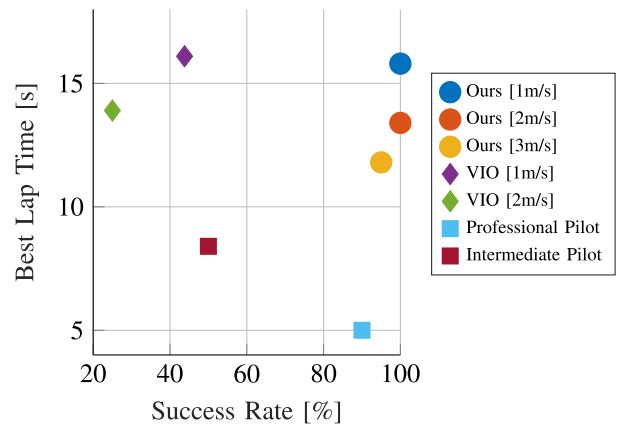
Fig. 12. Results on a real race track composed of four gates. Our learning-based approach compares favorably against a set of baselines based on visual-inertial state estimation. Additionally, we compare against an intermediate and a professional human pilot. We evaluate success rate using the same metric as explained in Section IV-B.
