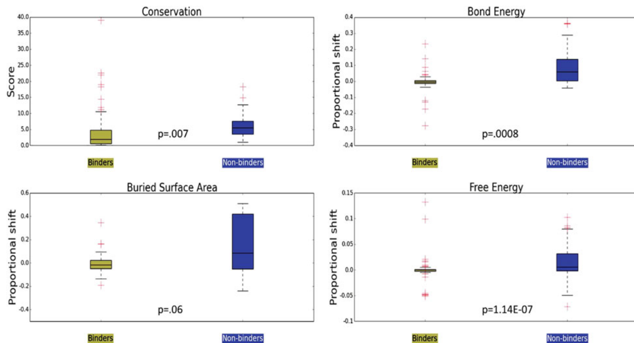
Fig. 4. Boxplots of values for features used in model. Binders and non-binders are shown in tan and blue, respectively, while outliers are indicated by red plus signs.
