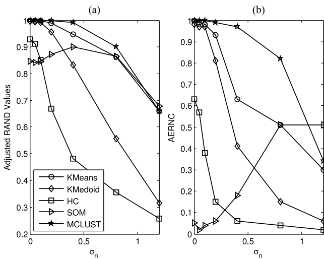
Fig. 4. Results for S1 data sets: (a) ARI versus \sigma_n for five clustering algorithms when K = 11 . (b) AERNC versus \sigma_n of ARI for five clustering algorithms.
