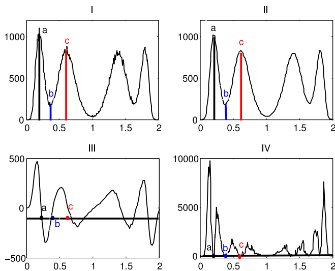
Fig. 2. The process to calculate the bounds of \alpha and \beta . (I) Dissimilarity distribution of the synthetic gene data set and points a, b and c are what we need to find out to calculate the bounds. (II) The smoothed distribution curve filtered by a rectangular window with the size of 10. (III) The derivative of the distribution function. (IV) A methods to find the zero points in the derivative of the distribution function.
