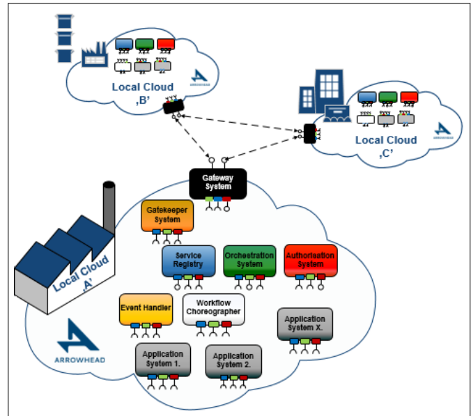
Fig. 2. Generic example of using intercloud servicing within Arrowhead.
