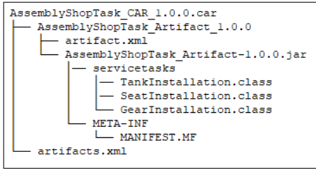
Fig. 9. Tree structure of CAR artifact.
